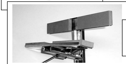
PINZA MECCANICA INOX ( A MOLLA) MECHANICAL CLAMP INOX ( by SPRING) PINCE MECHANIQUE ( à RESORT )
